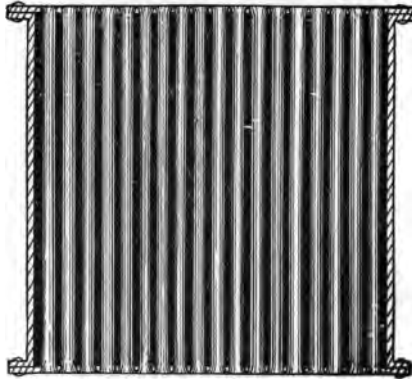
FIG. 34.—Copper Shell and Flue Boiler, with flange connections for the tube plates, as used on the "Locomotive" and other American steam carriages. The shell is strengthened by winding several layers of steel piano wire around the length of the boiler. This cut gives a section on the centre, showing one row of flues.
